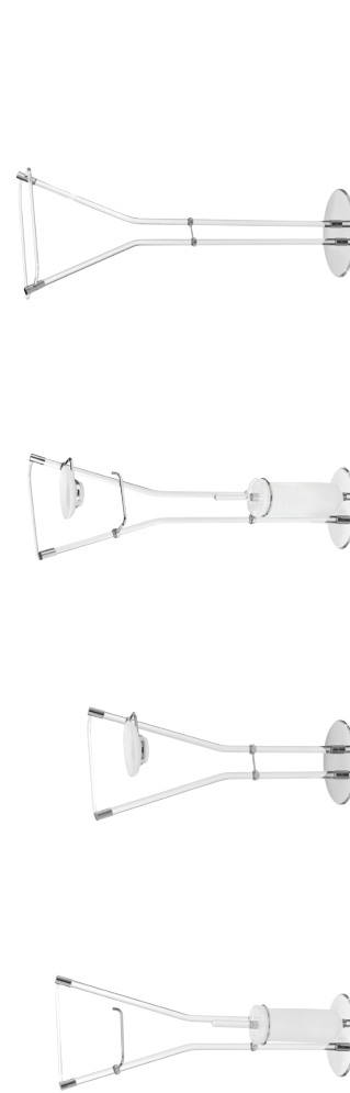
BASE PLEXIGLASS/PLEXIGLASS BASE K 159 Piantana portariviste, base plexiglass Vertical magazine stand, plexiglass base Base Ø 225 L. 235 H. 710 mm
